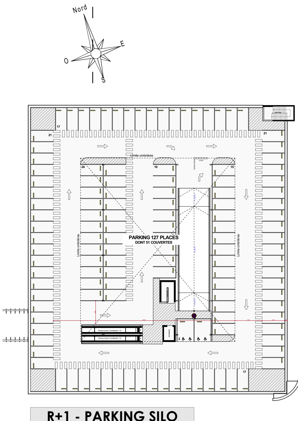
R+1 - PARKING SILO
