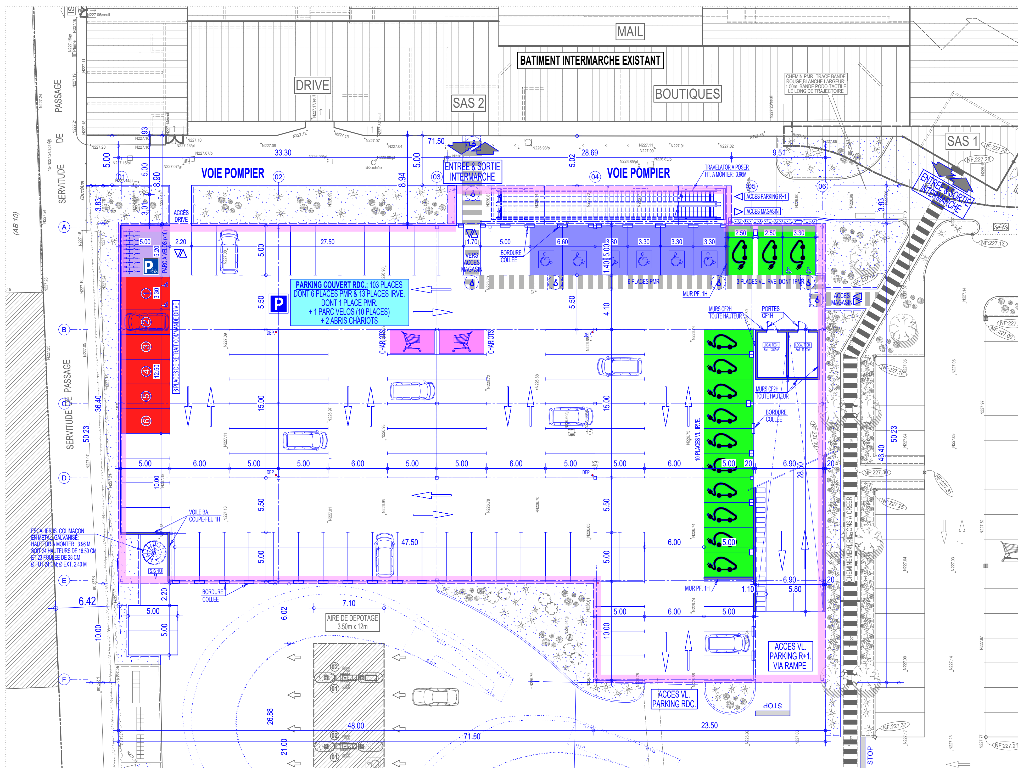
PLAN PARKING REZ-DE-CHASSEE - ECHELLE: 1/200
