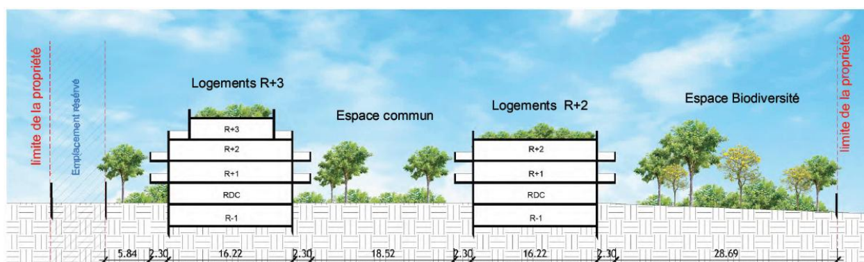
Figure 6: Coupe de principe
