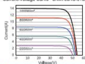
Current-Voltage Curve JAM78D40-610/MB
